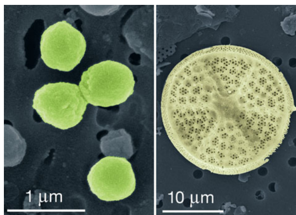
False color SEM of cyanobacteria, Prochlorococcus spp. (left), and a fossil centric diatom, Actinocyclus spp. (right).
