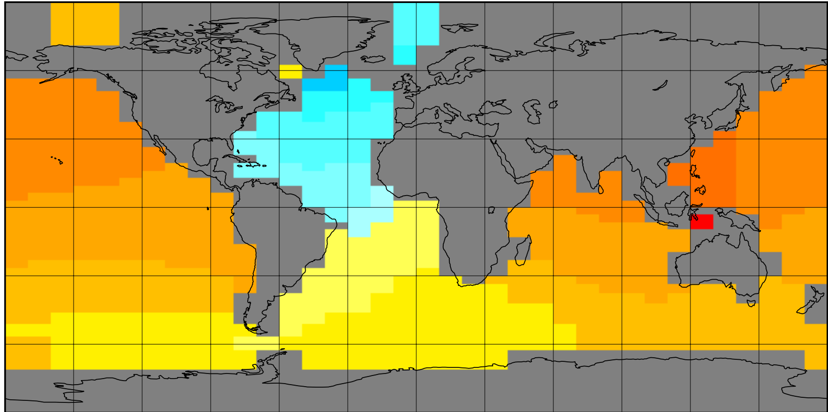
dissolved phosphate (PO4): 2106 m
