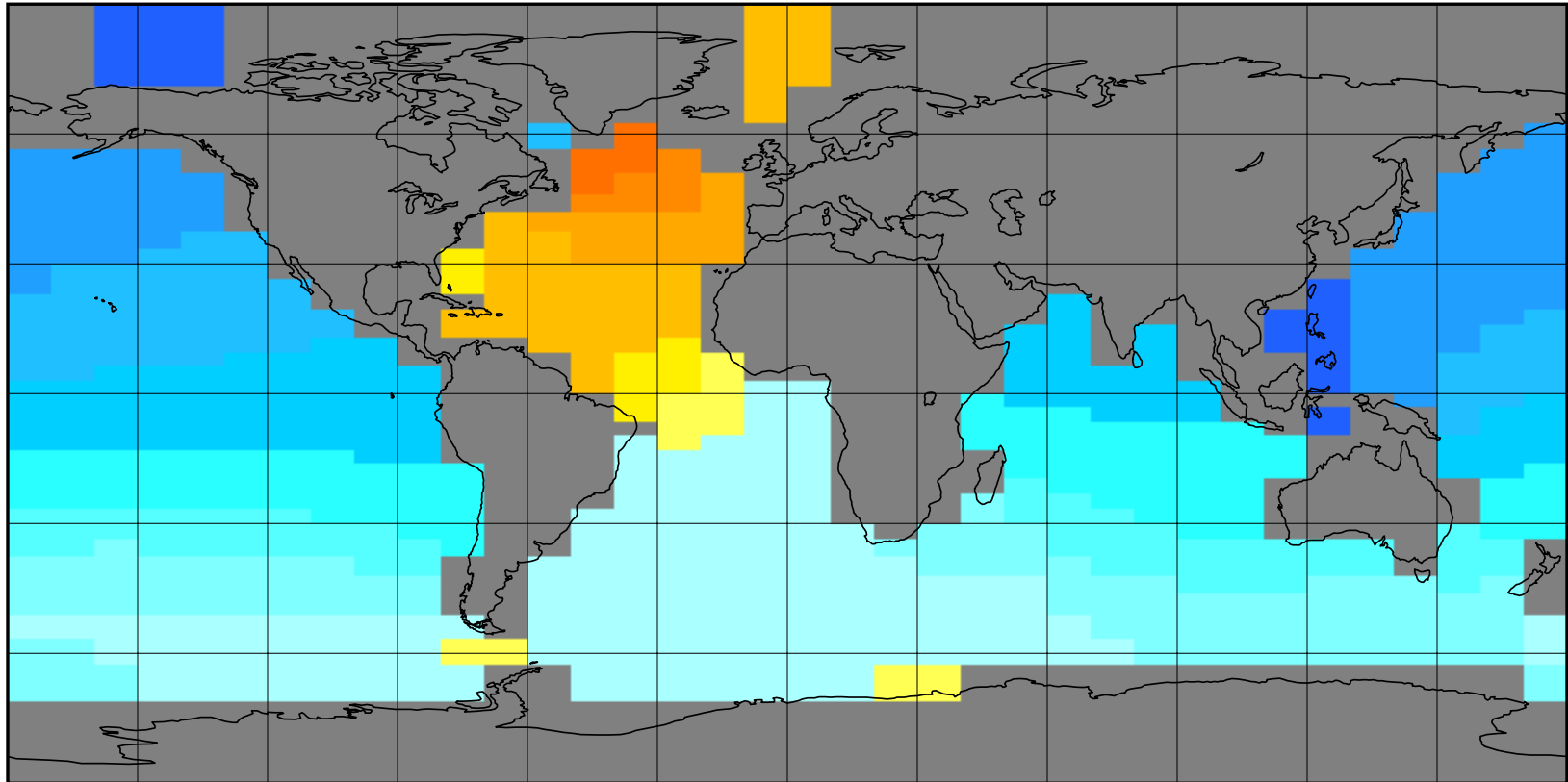
d13C of DIC: 2106 m
